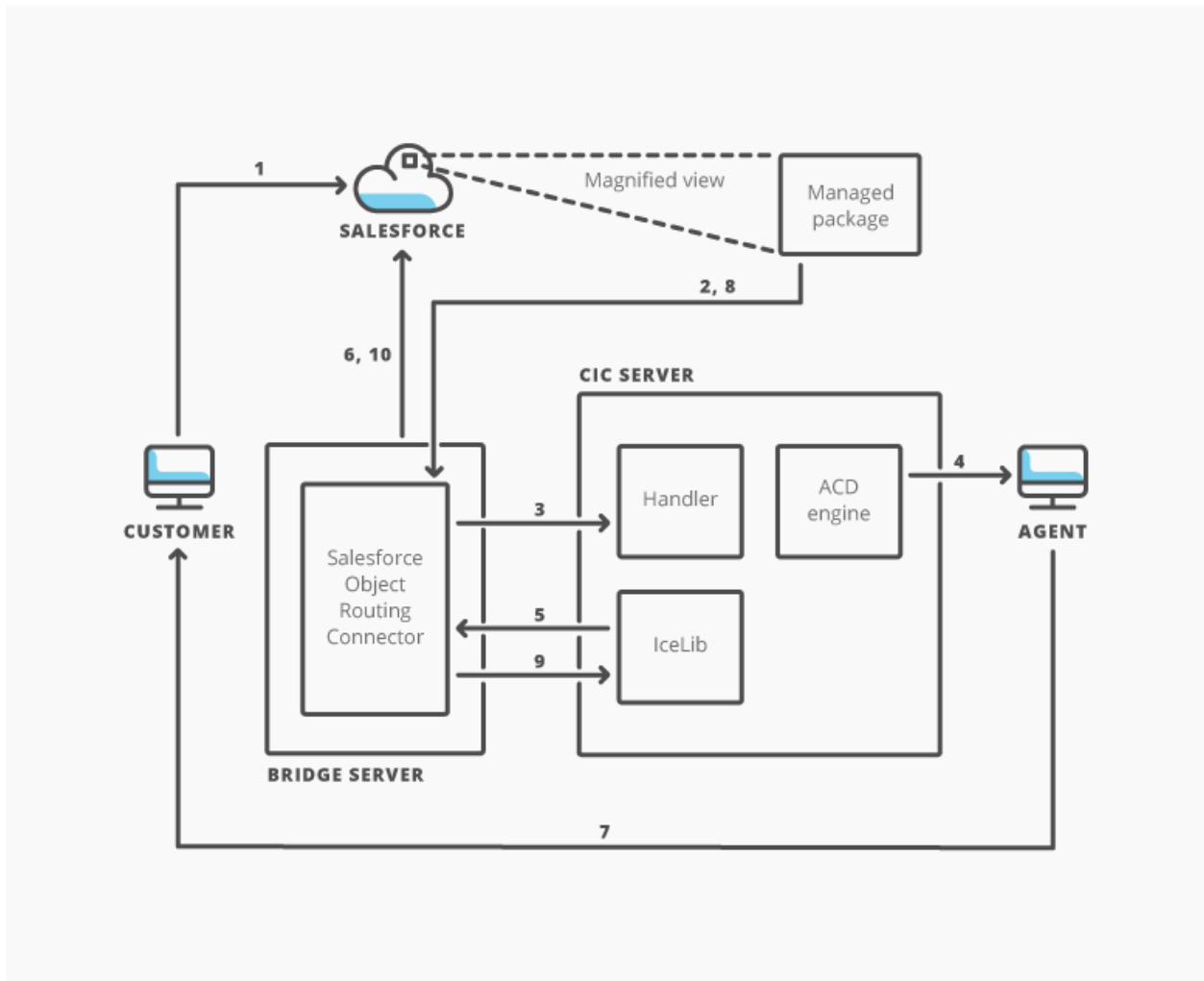
Workflow for the Salesforce Object Routing Connector
