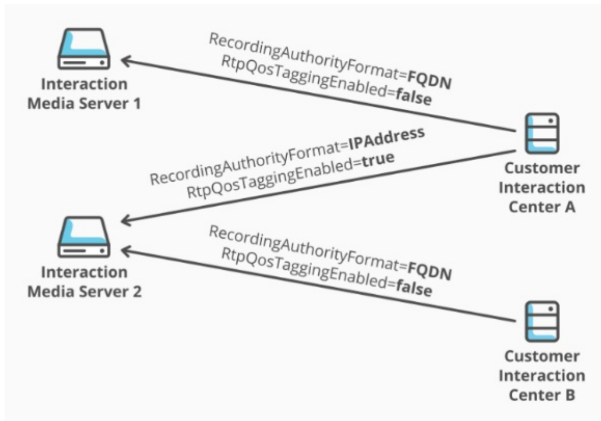
Interaction Media Server property override hierarchy
